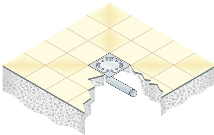
FLOOR FITTING LAYOUT OF A LATERAL DISCHARGE ICxP 20L DRAIN COVER
