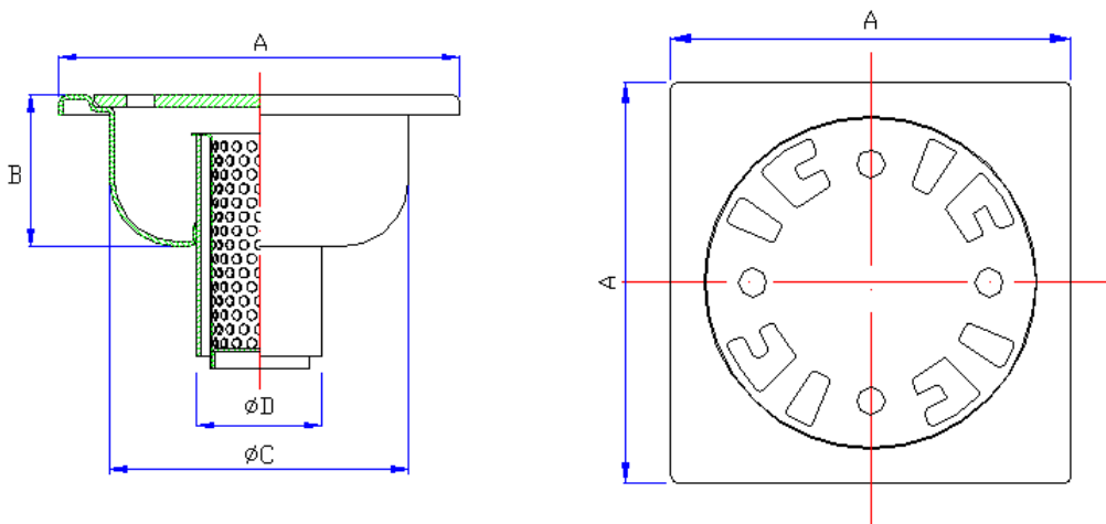
TECHNICAL DRAWING OF THE ICxP 20V DRAIN COVER WITH VERTICAL DISCHARGE
